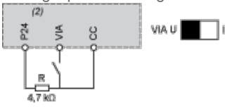
(2) ATV 212 control terminals
