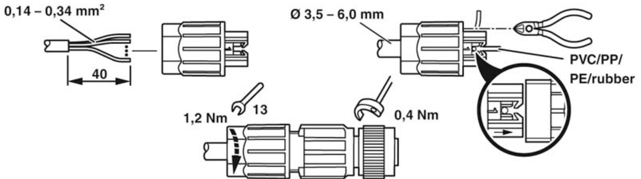
Functional drawing
