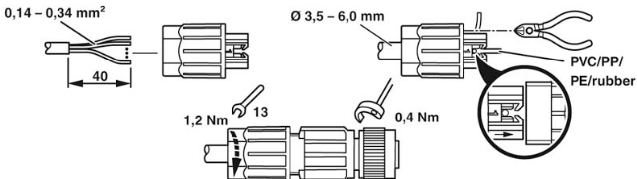
Functional drawing
