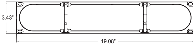
2RU, Cable Manager
