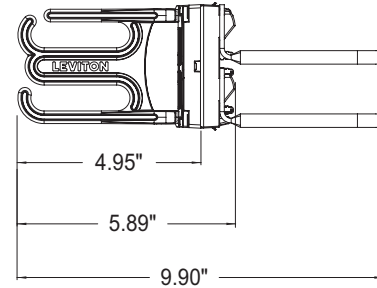
Side view, with front and rear cable managers attached
