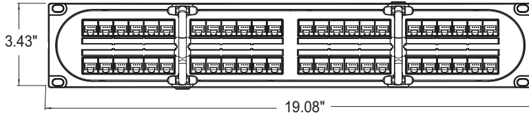
2RU, 48-port 110-style Patch Panel, Cat 5e
