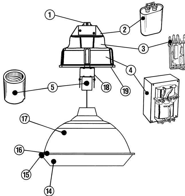
UM5 UNIMOUNT® 400 LUMINAIRE (Gen 5)
