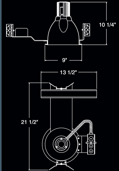
8" H.I.D. Downlight Height: 10 1/4" Ceiling Opening: 8" Trim O.D.: 9"
