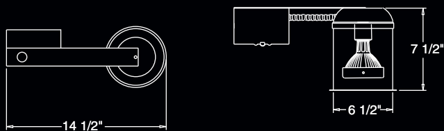
6" Adjustable H.I.D. Downlight, Electronic Height: 7 1/2" - Ceiling Opening: 6 1/2" - Trim O.D.: 7 1/4"
