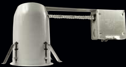
ELR4M20E 20W, M156, MR16, GX10 base, 120V Electronic Ballast, Remodel housings
