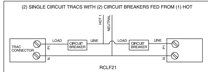
Diagram 4 (In-Line Feed)
