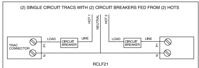
Diagram 4 (In-Line Feed)
