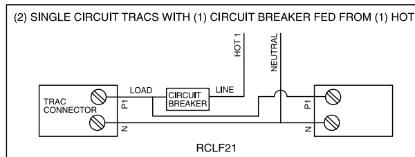
Diagram 2 (In-Line Feed)
