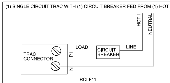
Diagram 2 (In-Line Feed)
