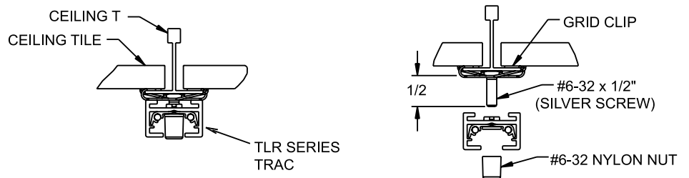
Figure 2 - TLVR Trac with a Flush Tile
