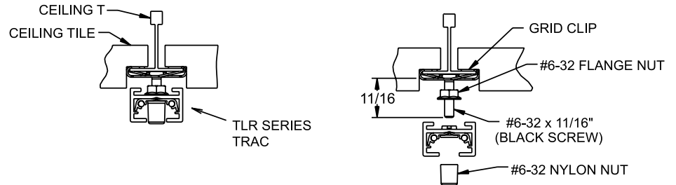
Figure 1 - TLVR Trac with a Drop Tile
