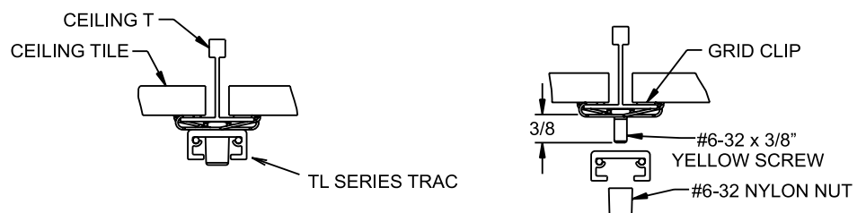
Figure 4 - TLV Trac with a Flush Tile
