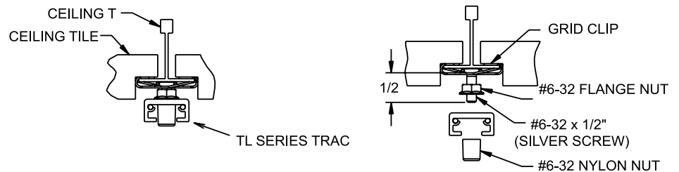
Figure 3 - TLV Trac with a Drop Tile
