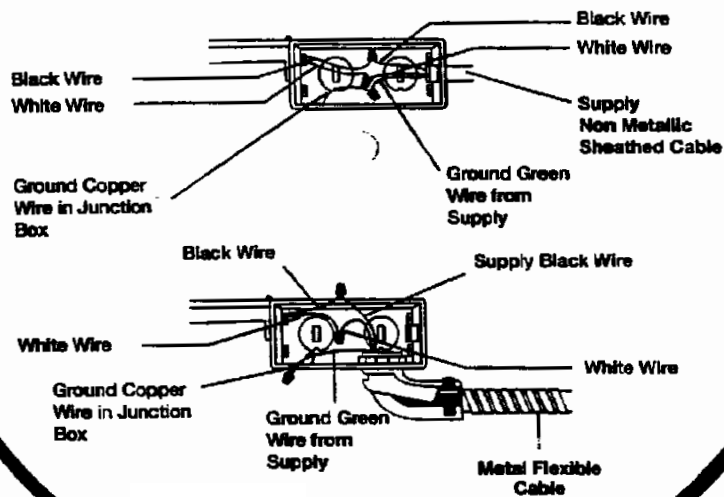
View with Junction Box Cover Off
