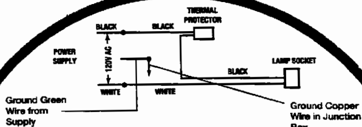
View with Junction Box Cover Off
