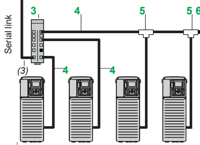
Example of serial link architecture
