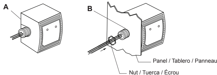
Figure / Figura / Figure 2 : Wiring / Alambrado / Câblage
