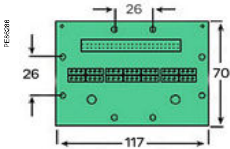
PowerLogic BCPM adapter board (one board per 21 split-core branch CTs)
