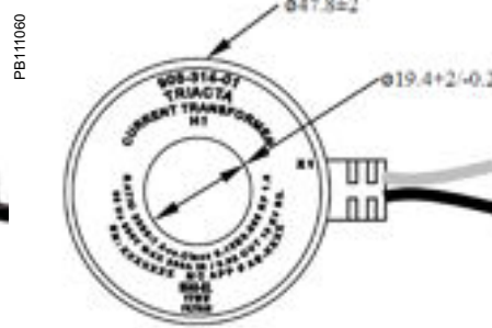
200 A CT dimensions
