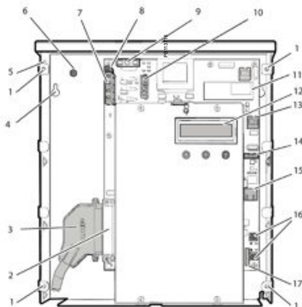
PowerLogic EM4033 and PowerLogic EM4080 internal view
