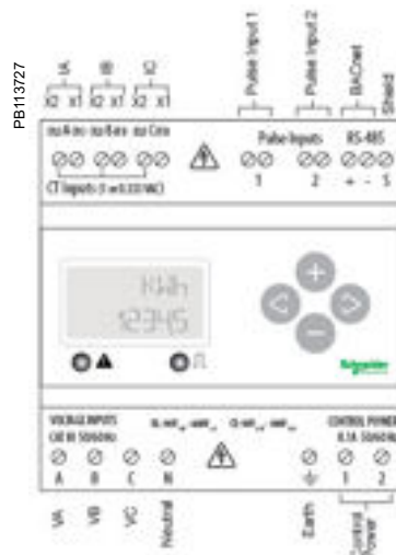
EM3500 parts and connection terminals
