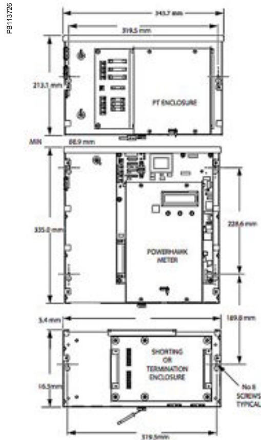
EM4X00, CT termination, PT module
