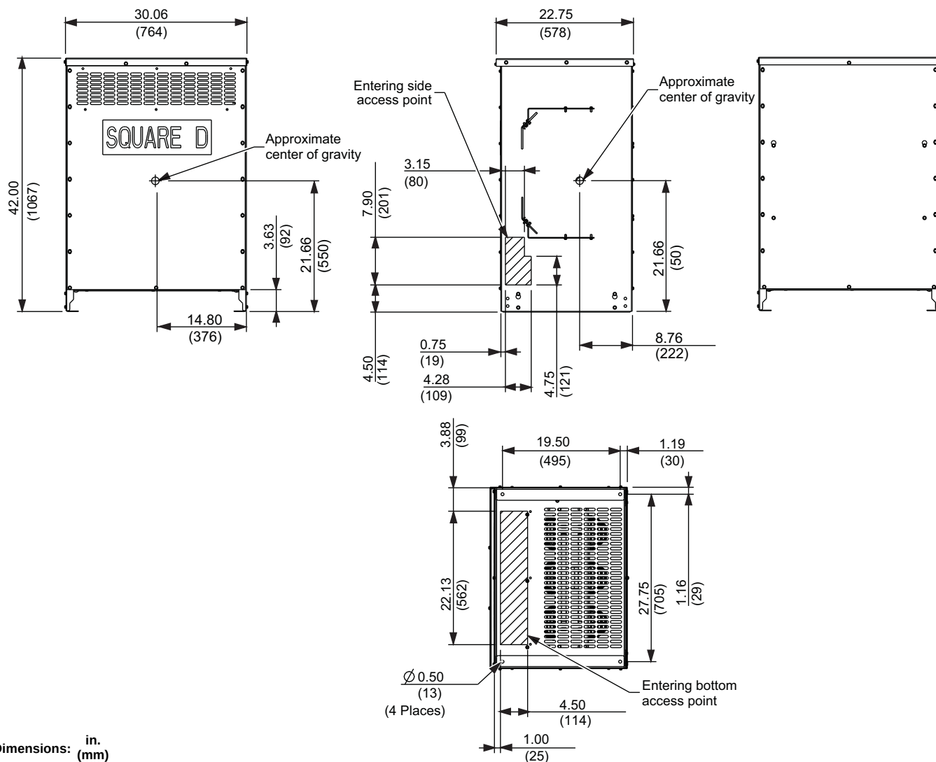
Figure 9: Enclosure 20K
