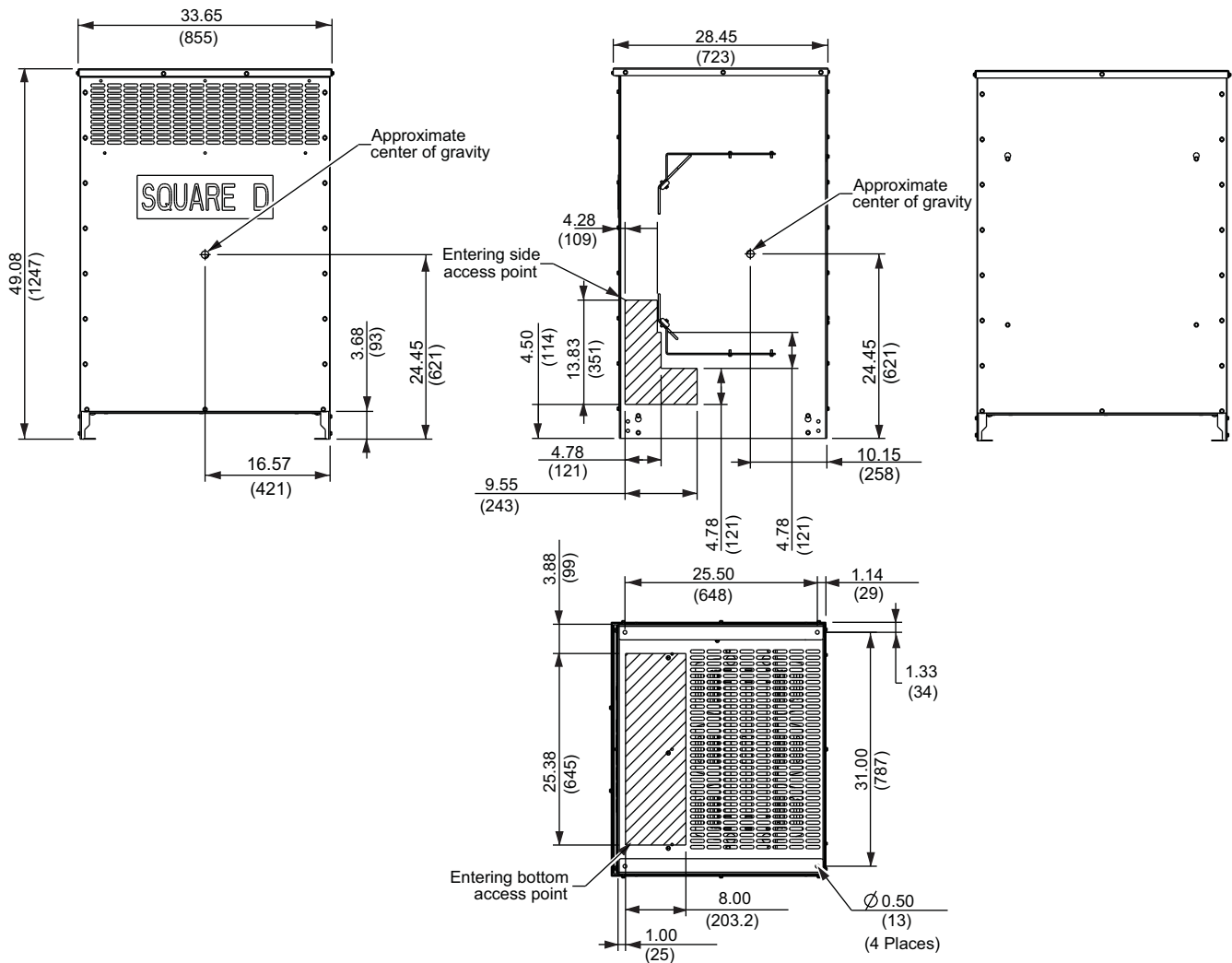
Figure 11: Enclosure 22K
