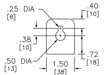
TOP MOUNTING BRACKET
