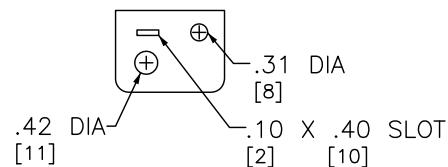
SEAL BRACKET
