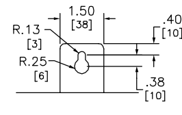
DETAIL C TOP MOUNTING BRACKET
