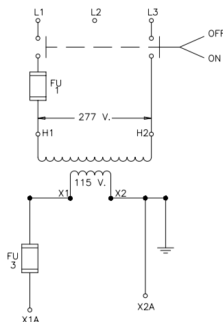
277 to 120, Voltage code D4
