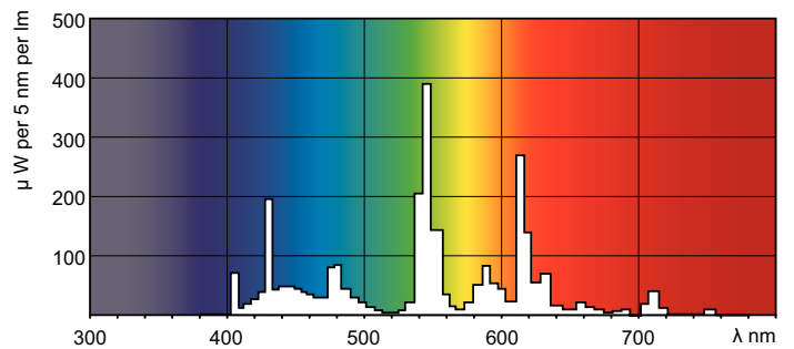
LDPO_TL5-HO8_850-Spectral power distribution Colour
