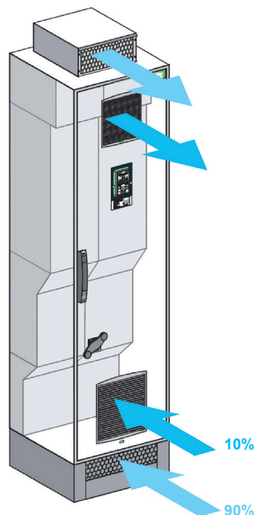
Type 12 cooling system
