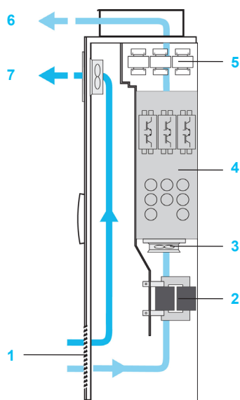
Type 1 enclosure
