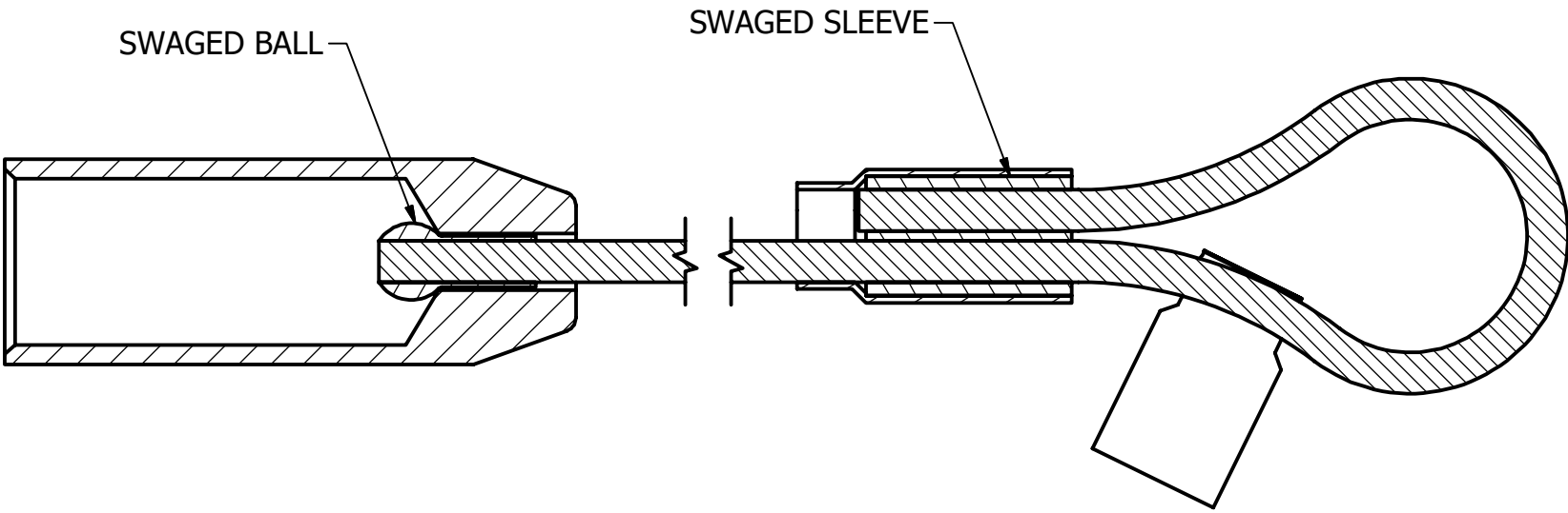
SECTIONAL VIEW
