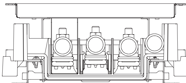
400 A Lugs Installed — NQCUV4
