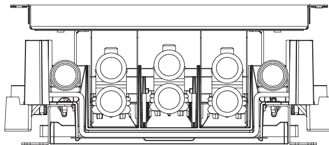
400 A Lugs Installed — NQALV4
