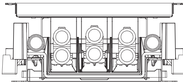
600 A Lugs Installed (NQALV6 and NQCUV6)
