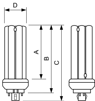
PL-T 42W/841/A/4P/ALTO
