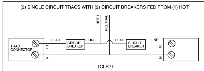
Diagram 4 (In-Line Feed)
