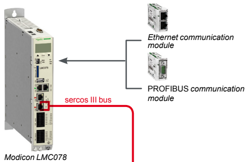
Modicon LMC078
