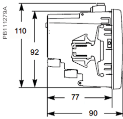
PM5500 / PM5600
