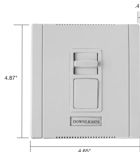
Dimensions for Wide Devices
