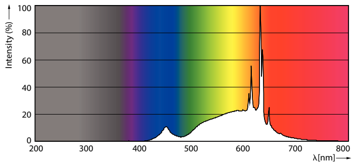
LEDBulbs_R20 120V 5-45W 450lm 90D 2700-2200K E26
