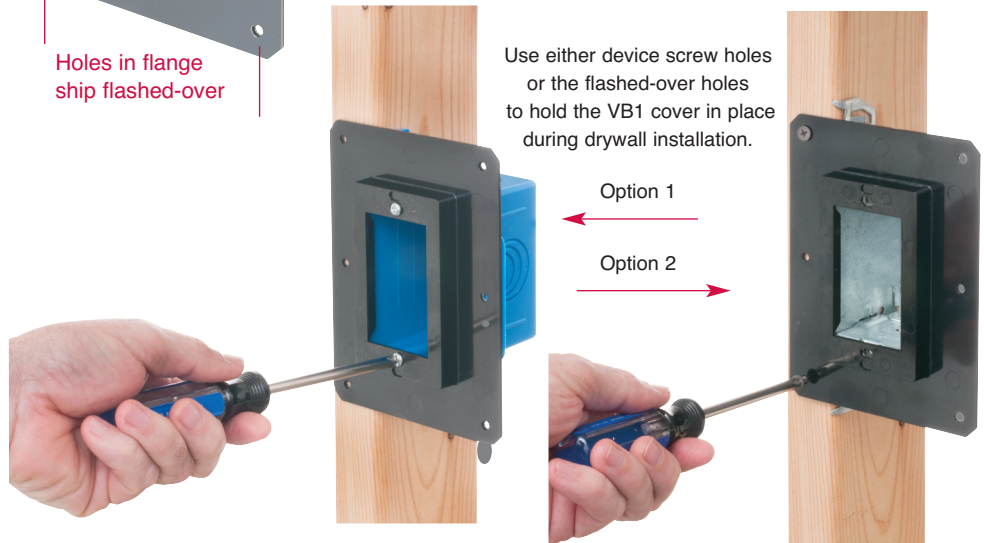
VB1 covers a plastic or steel single gang box.
