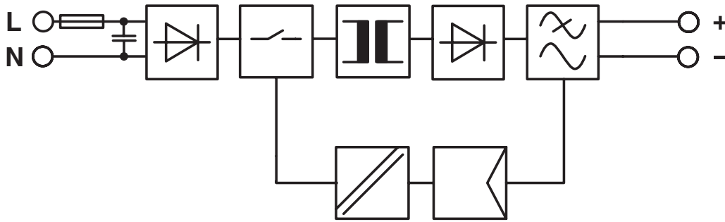
Block diagram
