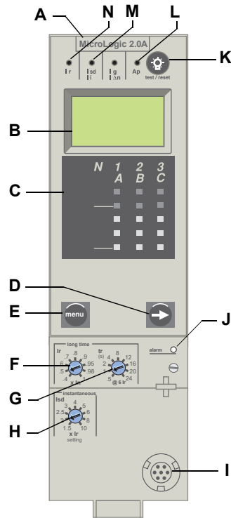
Figure 2 – 2.0A Trip Unit
