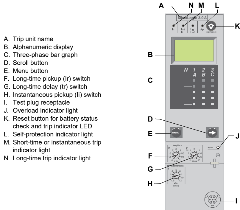
Figure 3 – 3.0A Trip Unit
