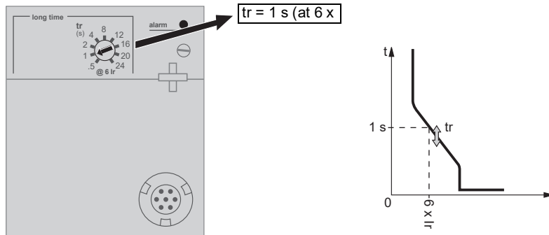
Figure 28 – Set Time Delay
