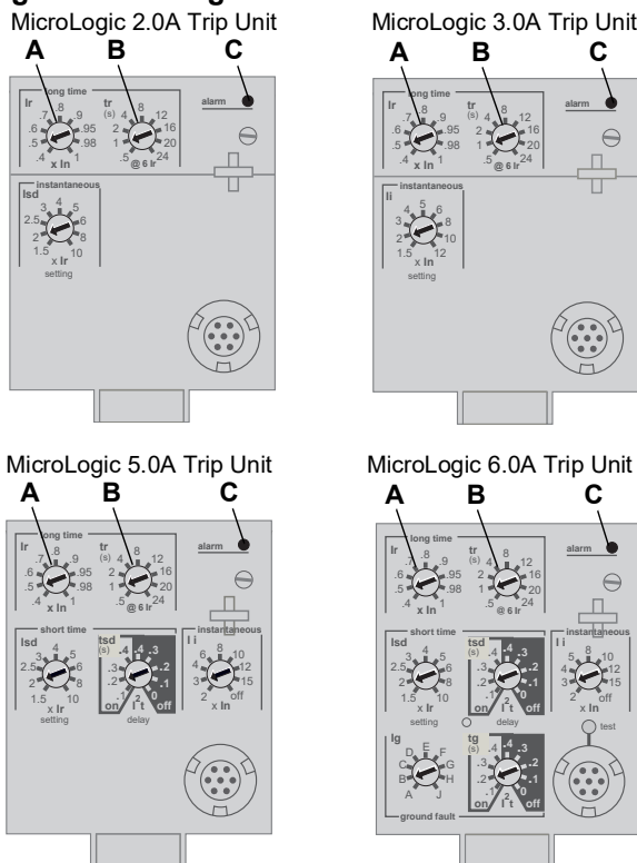
Figure 7 – Long-Time Protection Switches
