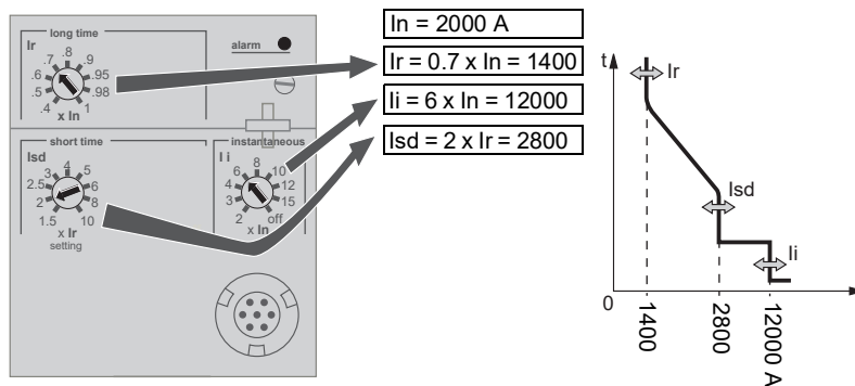
Figure 29 – Set Pickup Levels
