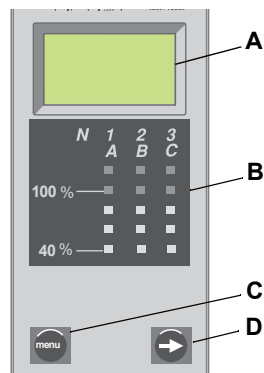
Figure 14 – Ammeter
