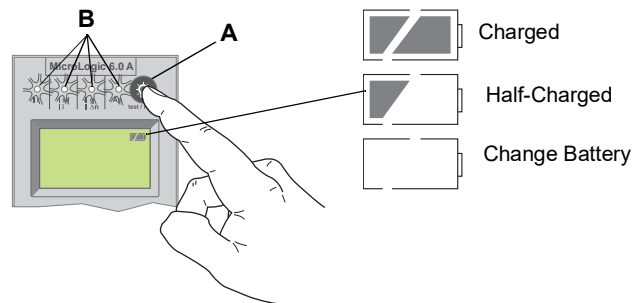
Figure 40 – Check Trip Unit Status
