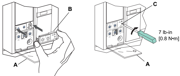
Figure 47 – Install Adjustable Rating Plug
