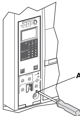
Figure 38 – Test Equipment Ground-Fault Trip Function
