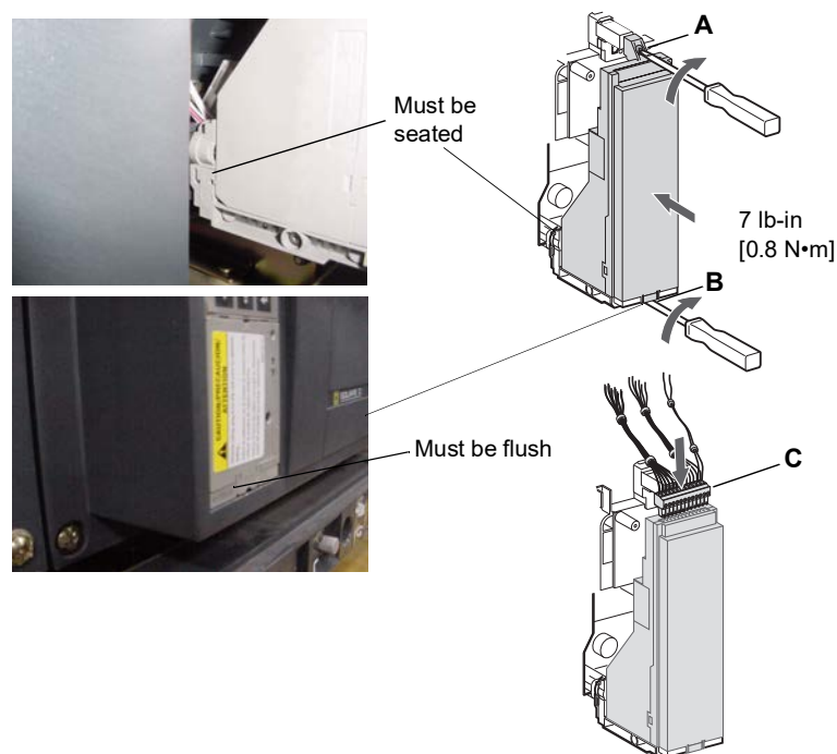
Figure 46 – Install Trip Unit
