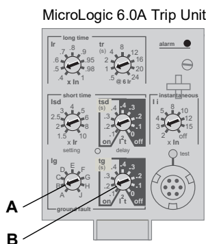
Figure 10 – Ground-Fault Protection Switches
