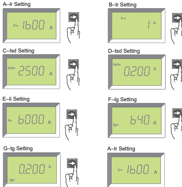
Figure 21 – Trip Unit Switch Settings
