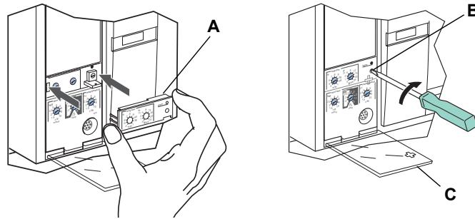
Figure 49 – Install New Adjustable Rating Plug
