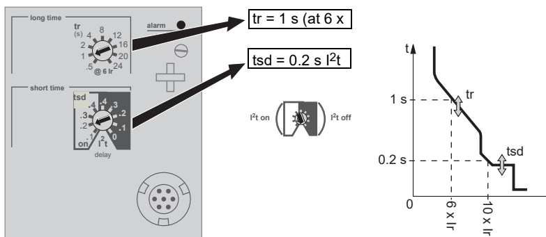
Figure 30 – Set Time Delays
