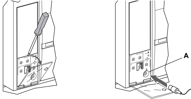
Figure 37 – Verify Trip Unit Operation
