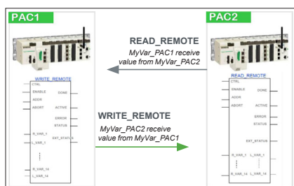
Explicit messaging
