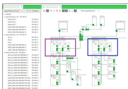
Implicit messaging
