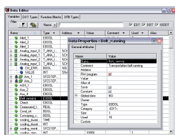
Data properties
