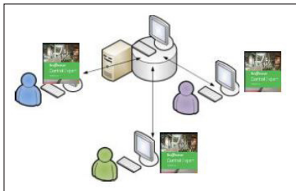
Client-Server model
