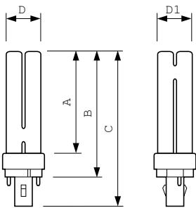
PL-C 18W/841/2P/ALTO 10PK
