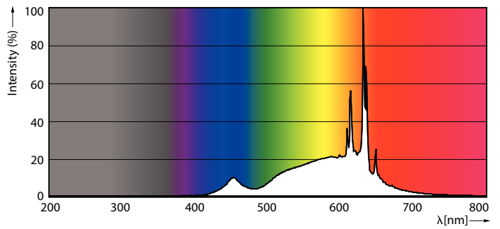
60W E26 A19 927 Frosted
