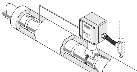
ECW-GF using RayClic power connection kit
