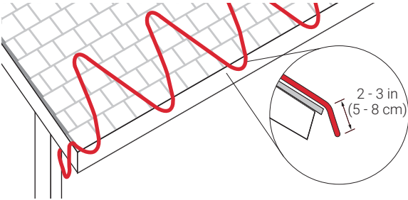
Figure 8: Layout for heated drip loops
