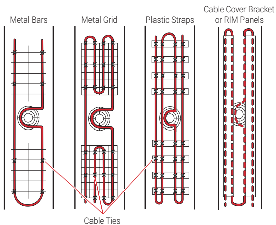
Installation of GM-XT cable in trench drains using metal bars/grids, plastic strapping and Cable Cover Bracket or RIM Panels system
