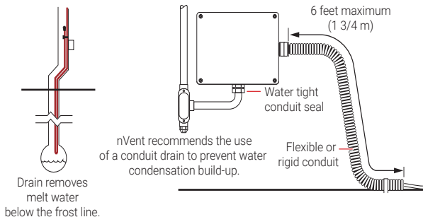
Figure 14: Installation of IceStop cable in trench drains
