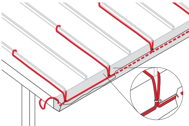
Figure 6: Layout on a standing seam room
