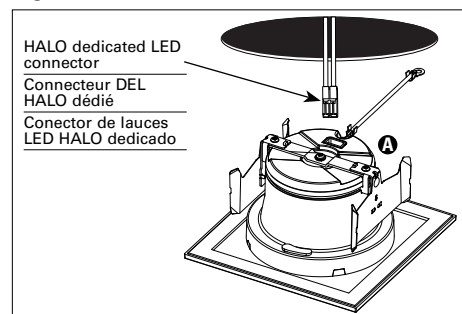
Figure 7. LED Connection
