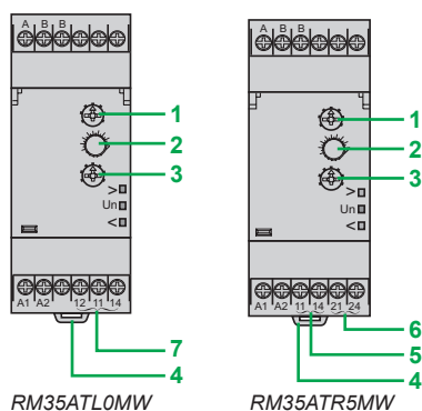
RM35ATL0MW
