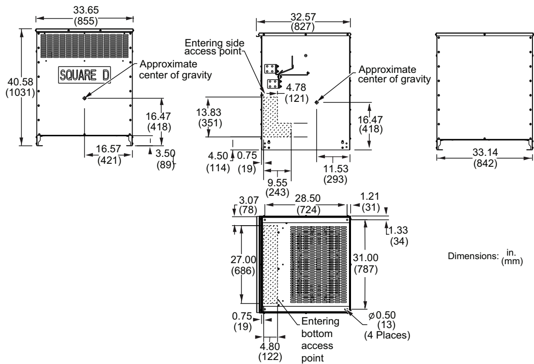
EXN150T3H Dimensions
