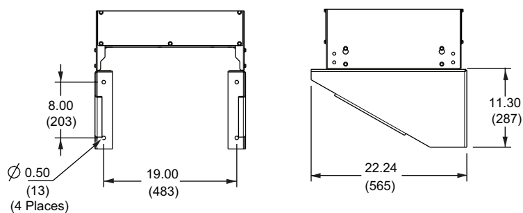
Wall Mounting Bracket: 7400WMB17M
