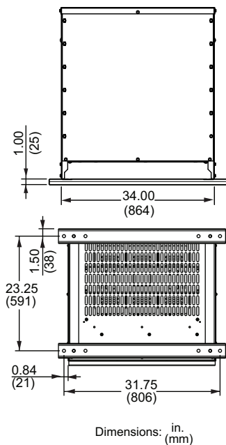
Ceiling Mounting Bracket: 7400CMB18M19M20M
