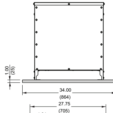
Ceiling Mounting Bracket: 7400CMB18M19M20M
