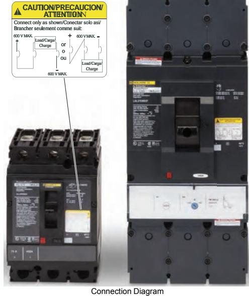
Connection Diagram
