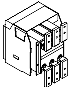
P-Frame Drawout Cradle Connections
